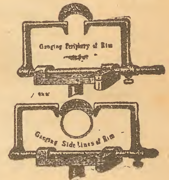
Wheel Truing Stand
